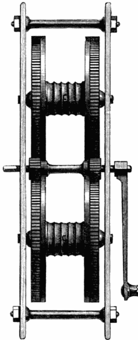
FIG. 52: ANOTHER FORM OF DOUBLE-BARRELLED CRAB
