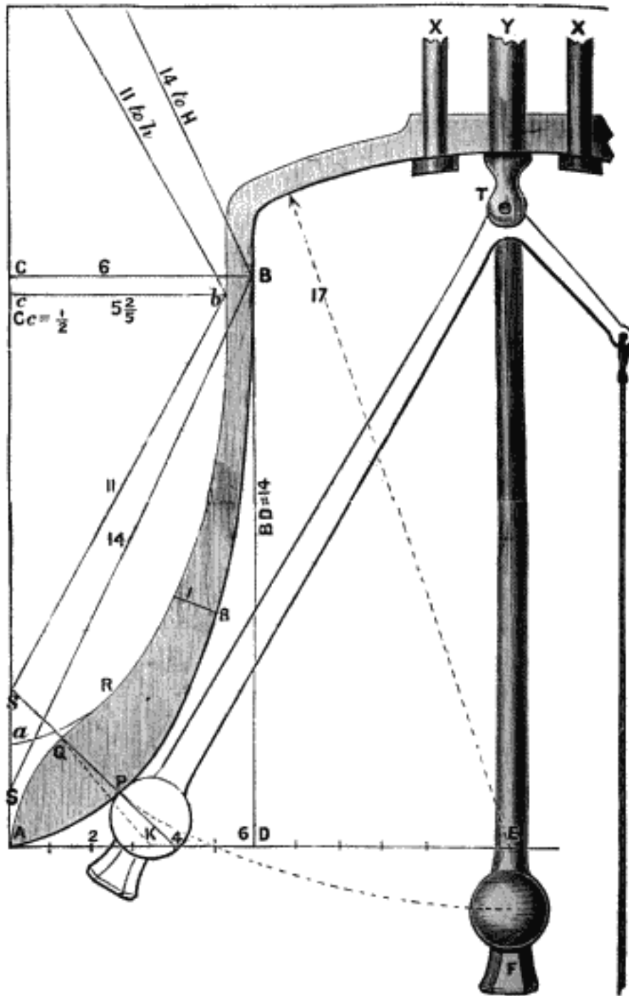
FIG. 80: 'SWEEP' OR SECTION OF A BELL
