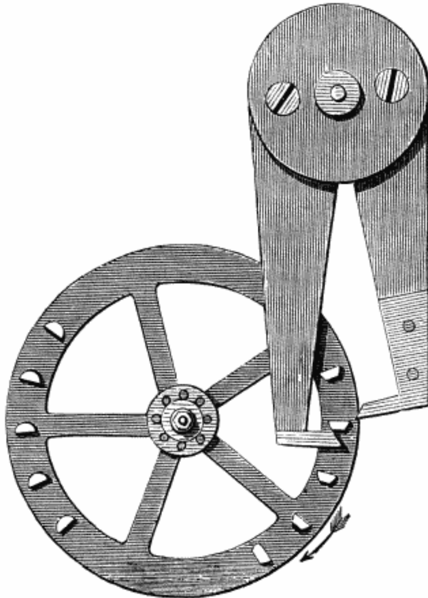
FIG. 15: PIN-WHEEL ESCAPEMENT
