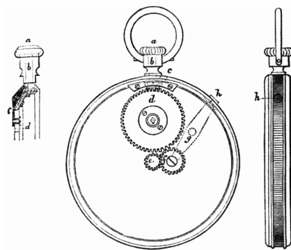
FIG. 78: KEYLESS WATCHES
